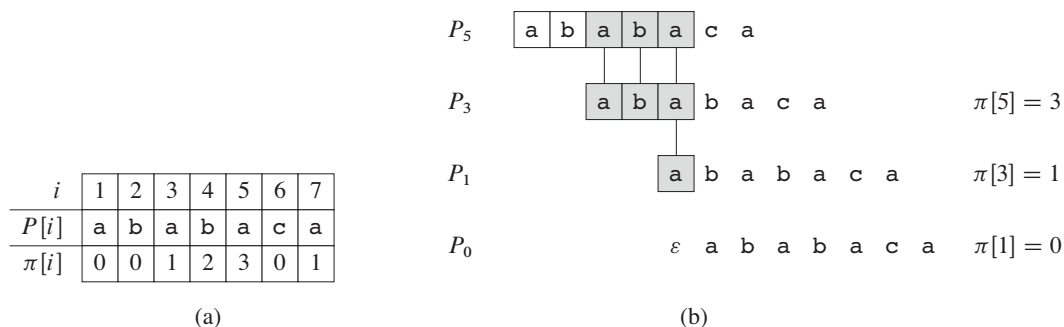
Figure 32.11 An illustration of Lemma 32.5 for the pattern P = ababaca and q = 5 . (a) The \pi function for the given pattern. Since \pi[5] = 3 , \pi[3] = 1 , and \pi[1] = 0 , by iterating \pi we obtain \pi^*[5] = \{3, 1, 0\} . (b) We slide the template containing the pattern P to the right and note when some prefix P_k of P matches up with some proper suffix of P_5 ; we get matches when k = 3, 1 , and 0 . In the figure, the first row gives P , and the dotted vertical line is drawn just after P_5 . Successive rows show all the shifts of P that cause some prefix P_k of P to match some suffix of P_5 . Successfully matched characters are shown shaded. Vertical lines connect aligned matching characters. Thus, \{k : k < 5 \text{ and } P_k \sqsubset P_5\} = \{3, 1, 0\} . Lemma 32.5 claims that \pi^*[q] = \{k : k < q \text{ and } P_k \sqsubset P_q\} for all q .
